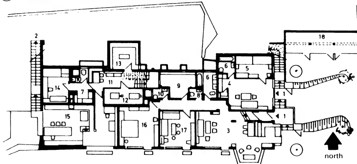
8 Ground floor
